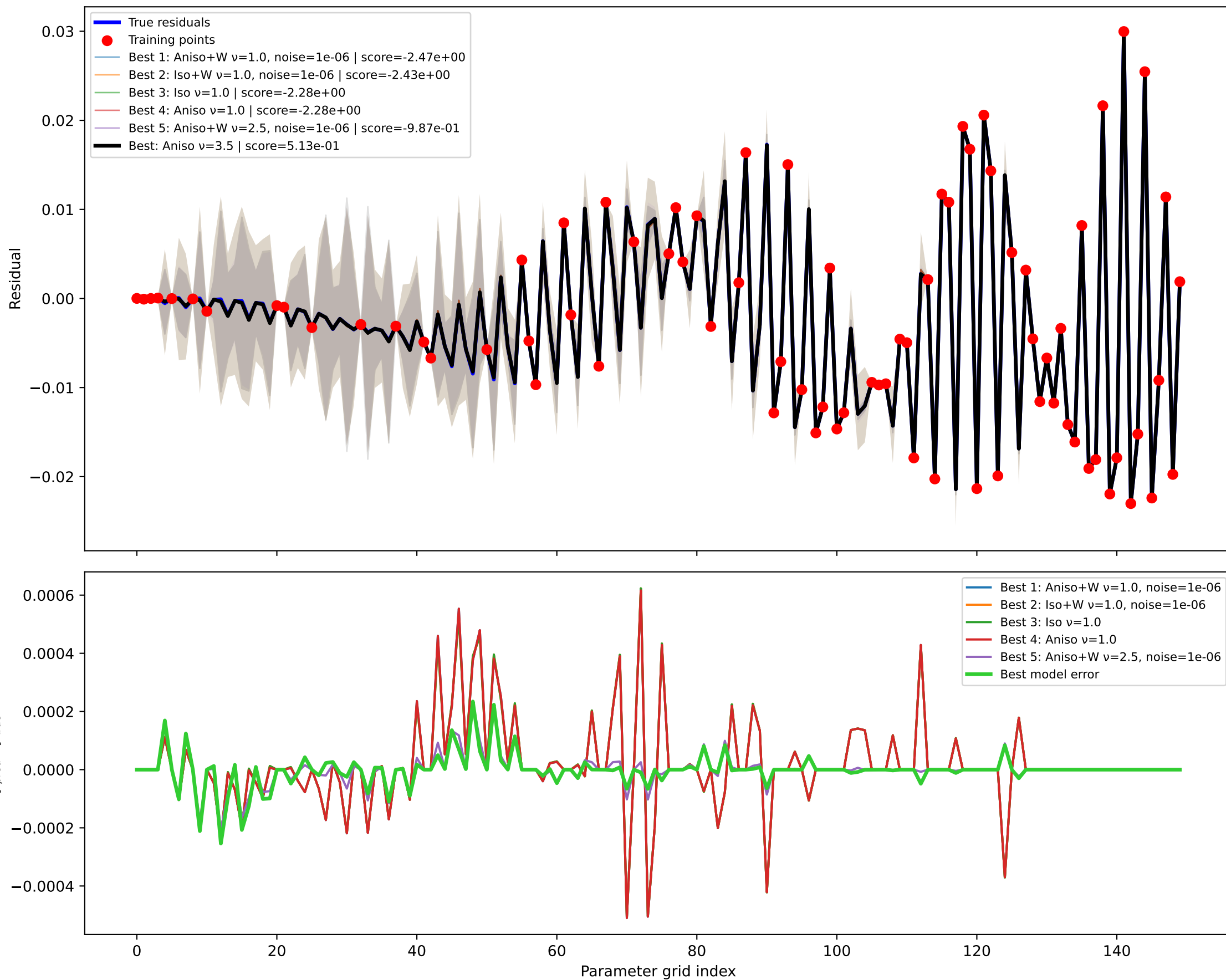
GPR kernel comparison node=27 RMSE=5.659e-05, train RMSE=1.676e-11
